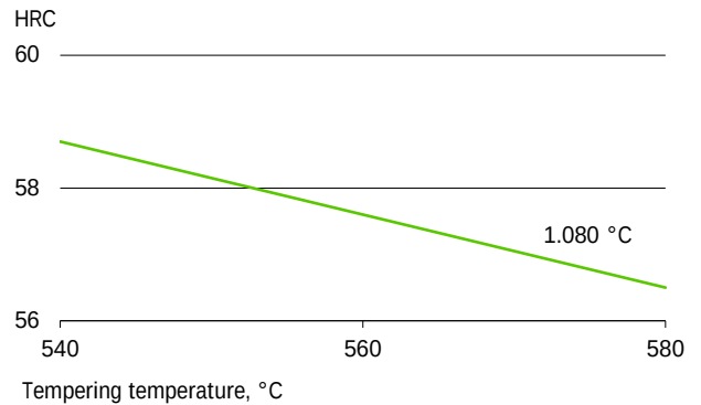
Tempering diagram (Hardness and Tempering)
